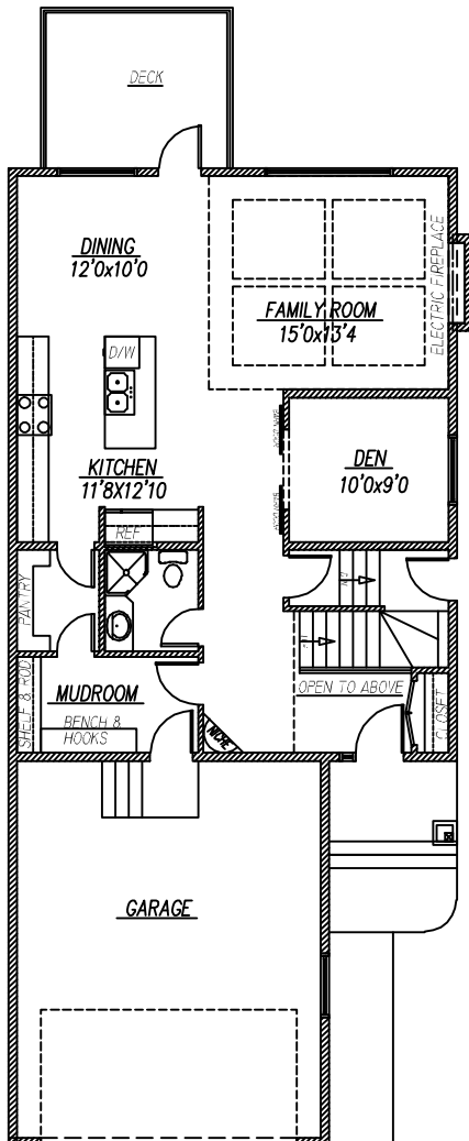
MAIN FLOOR PLAN 1042 SQ. FT.
